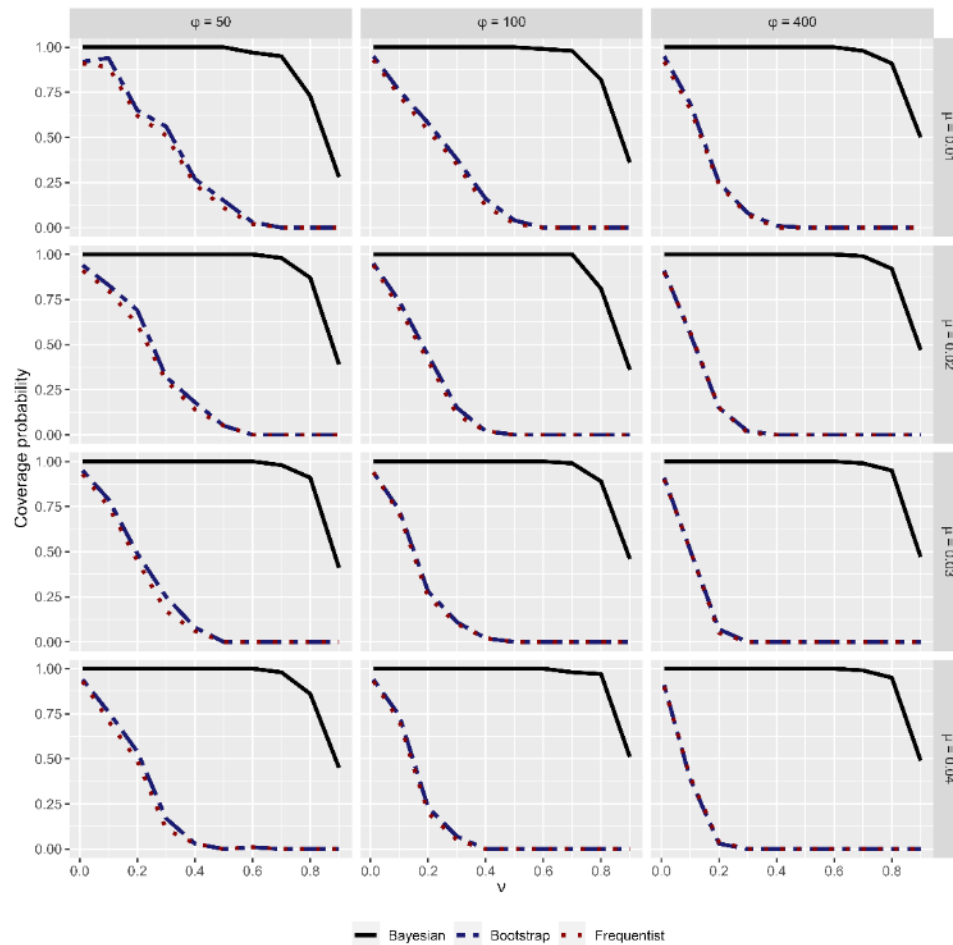
Figure 5 - Coverage probability of frequentist and bootstrap confidence intervals and credible intervals as a function of the v parameter of the BEZI distribution with \mu assuming values ranging from 0.01 to 0.04, \phi assuming values 50, 100 and 400 and v ranging from 0.1 to 0.9 for a sample size n = 60 .
